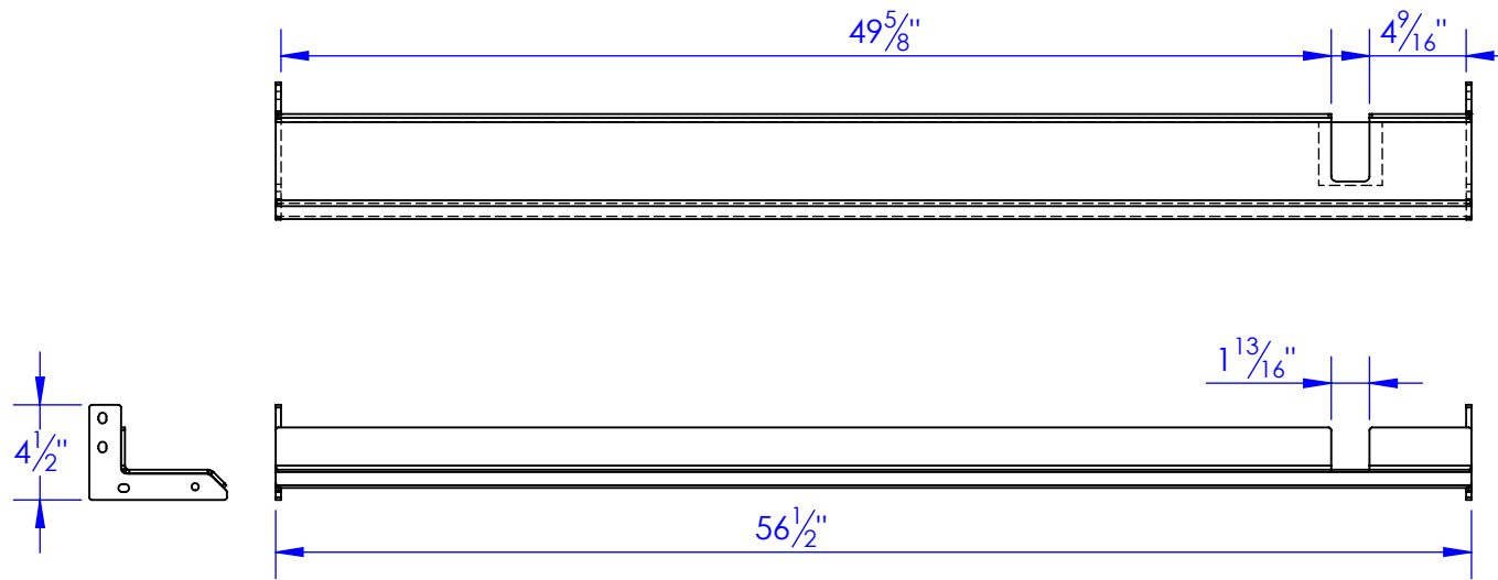
FP-FL9255-6 FENDER FLARE, PASS, FL9255, WLDMT DRAWING # 90-1205 QTY: 1
