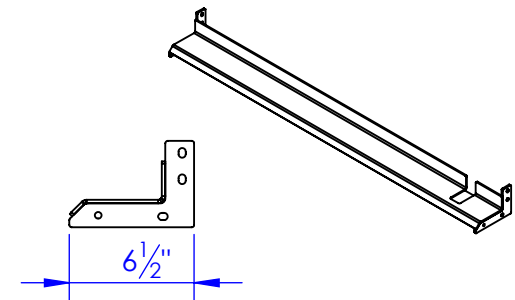
FP-FL9255-6 FENDER FLARE, PASS, FL9255, WLDMT DRAWING # 90-1205 QTY: 1
