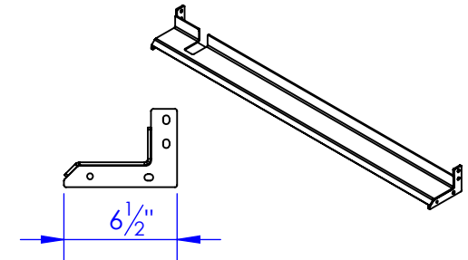
FP-FL9255-5 FENDER FLARE, DRIVERS, FL9255, WLDMT DRAWING # 90-1204 QTY: 1
